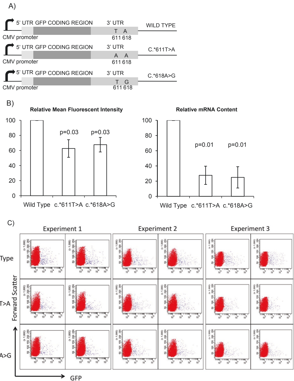
Figure 1 3'UTR plasmid reporter assay. A) Schematic diagram of pTH-GFP \alpha constructs used in mRNA translational efficiency assays. B) 3'UTR plasmid reporter system and FACS analysis (n = 3, duplicate wells analysed in each experiment, 2-tailed t-test, error bars SD); (i) Mean fluorescence intensity (MFI) of RT112 cells transfected with GFP-flanked by mutant 3'UTR sequences relative to that of GFP-flanked by wild-type XPC UTR sequences; (ii) Relative levels of GFP mRNA to 36B4 mRNA analysed by quantitative RT-PCR using the \Delta\Delta C_t method. C) Flow cytometry data of individual transfections (n = 3, duplicate wells analysed in each experiment). GFP fluorescence measured on x axis (forward scatter on y axis). See Table 3 for mean fluorescent intensity values.
